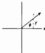
COSECANT cosecant \phi = \frac{1}{y}
