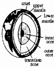
CORE cutaway view of earth
