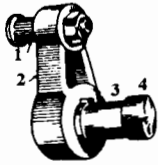
SINGLE OVERHUNG CRANK: 1 crankpin, 2 web, 3 journal, 4 crankshaft
