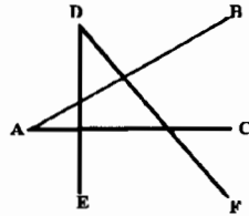
ANTIPARALLEL LINES (AB & AC are antiparallel TO DE & DF)
