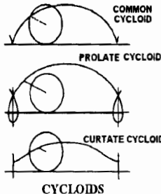
a cycloid curve
