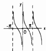
COTANGENT Graph of cotangent function: y = \cot x
