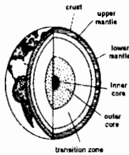
CRUST Cutaway view of Earth
